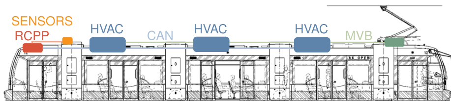
Fig. 1. Schematic of the tram.
