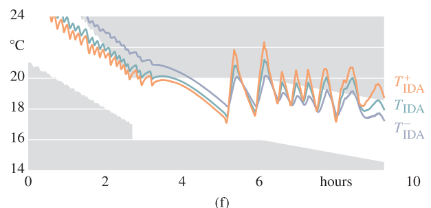
Fig. 6. Time series of the IDA temperature for individual tests.
