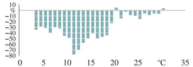
Fig. 7. Relative energy savings of the new tram (compared with the current tram) against the ODA temperature.
